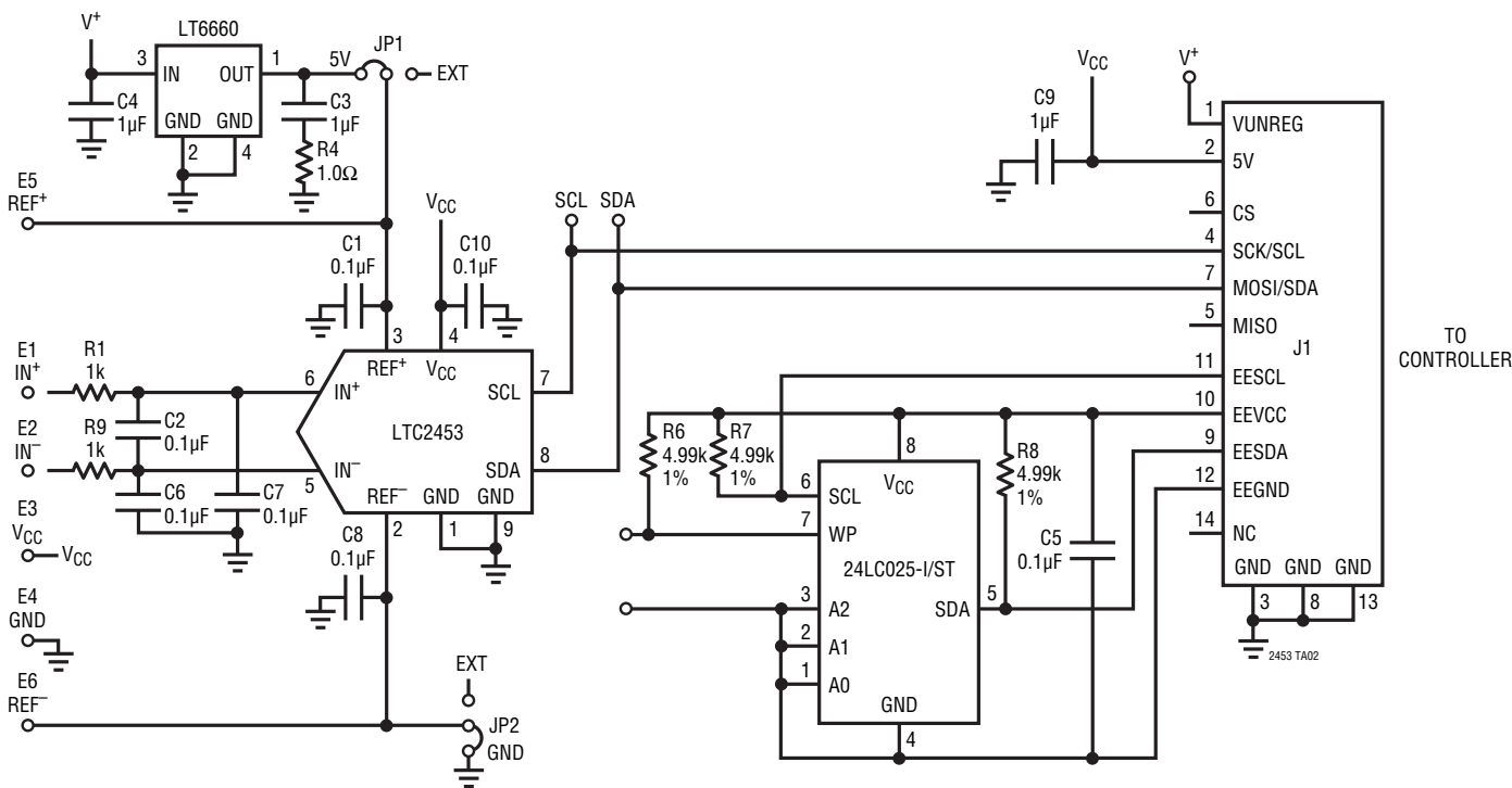
DC1266A Demo Board Schematic
